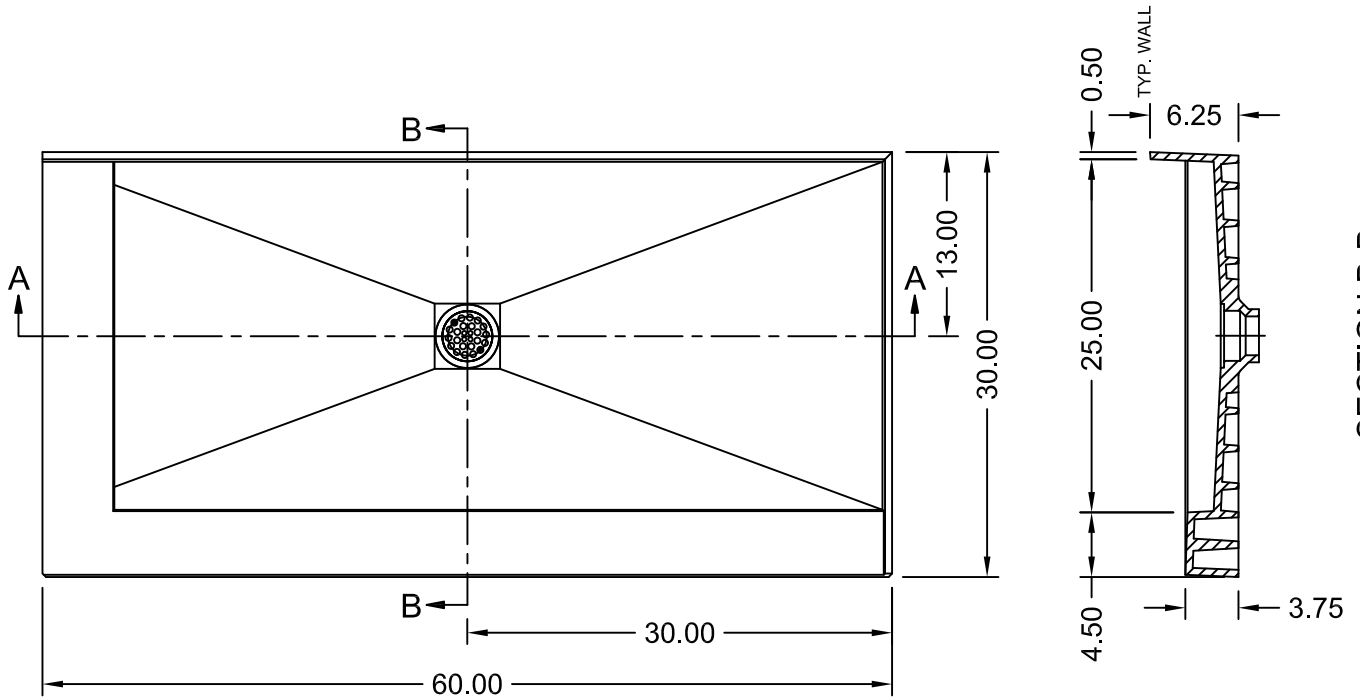
SECTION B-B
