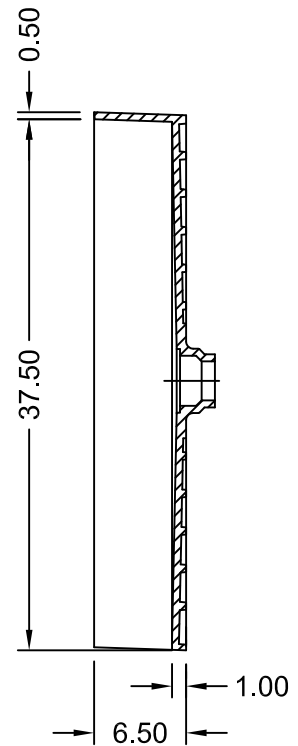
SECTION B-B
