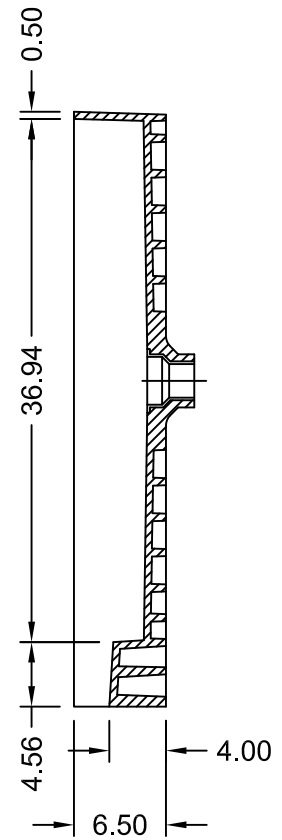
SECTION B-B
