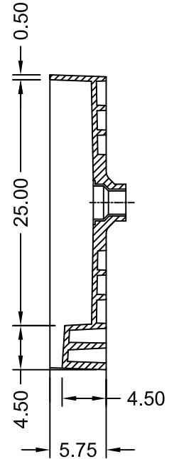
SECTION B-B
