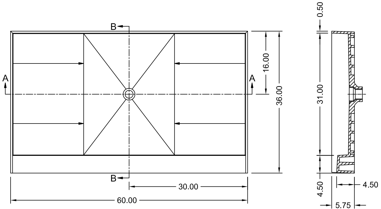
SECTION B-B
