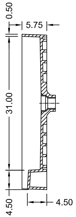
SECTION B-B
