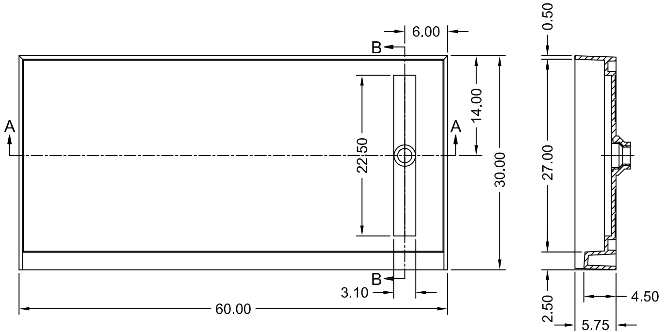
SECTION B-B
