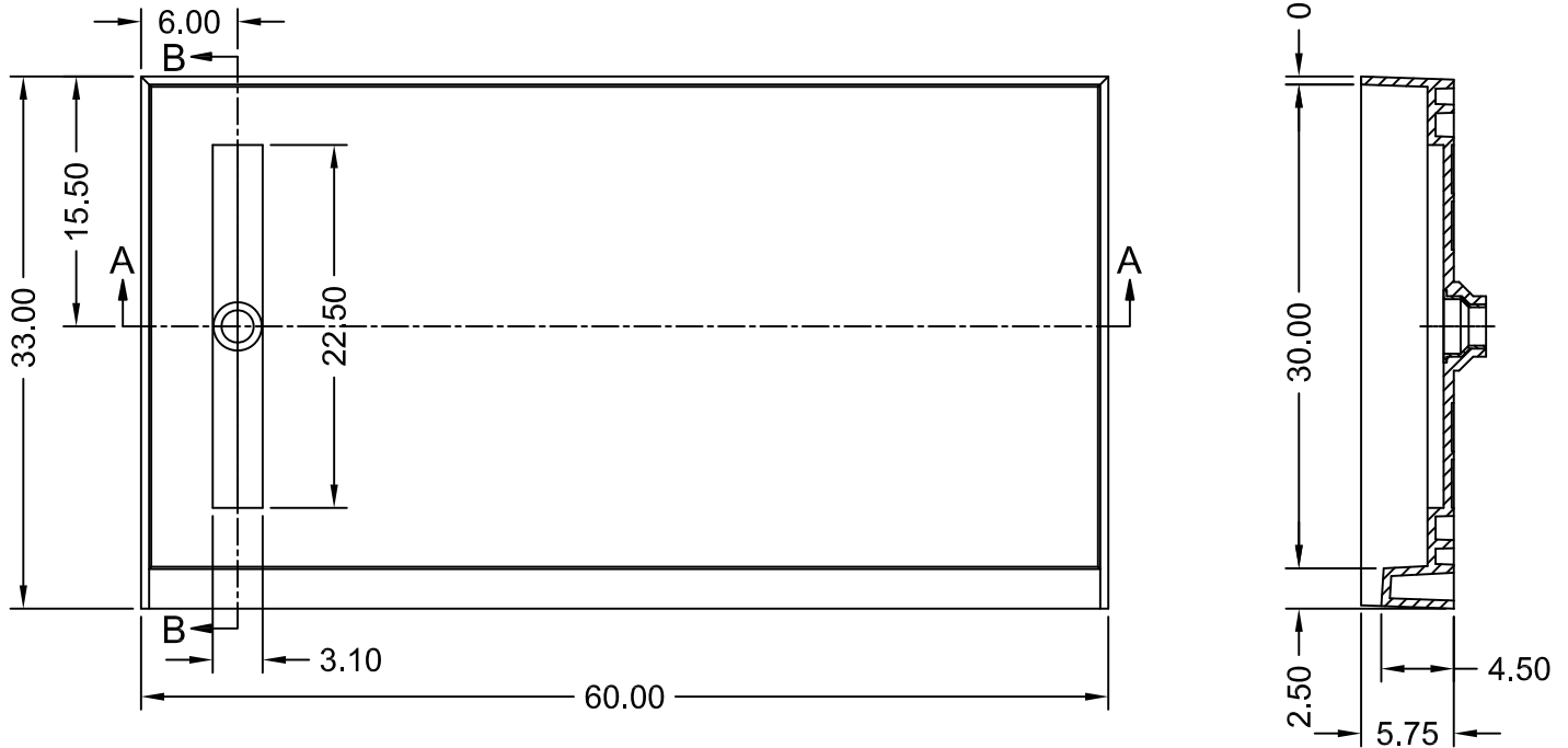
SECTION B-B
