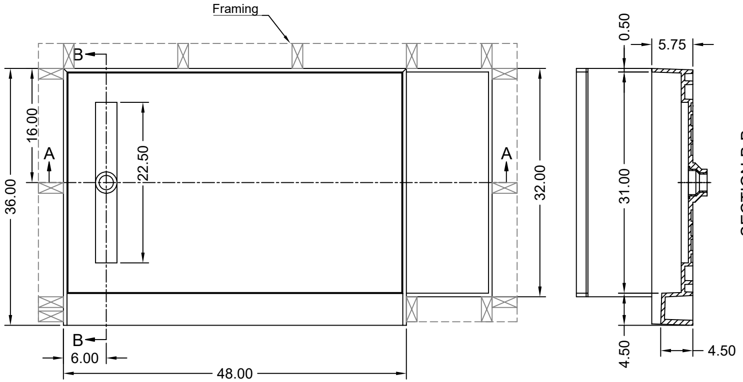
SECTION B-B
