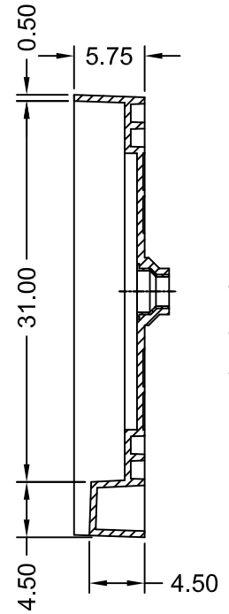
SECTION B-B
