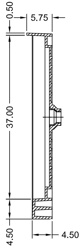
SECTION B-B
