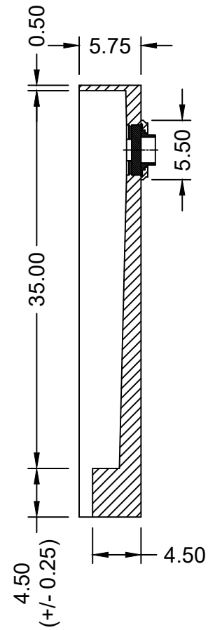
SECTION B-B
