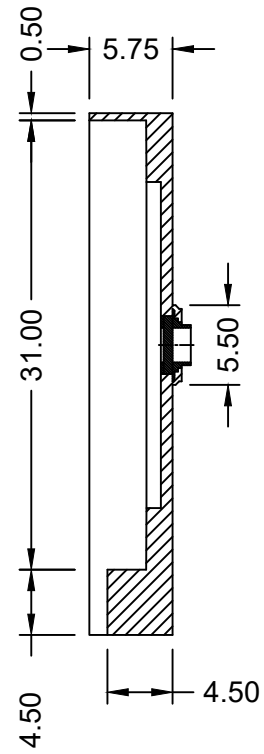
SECTION B-B
