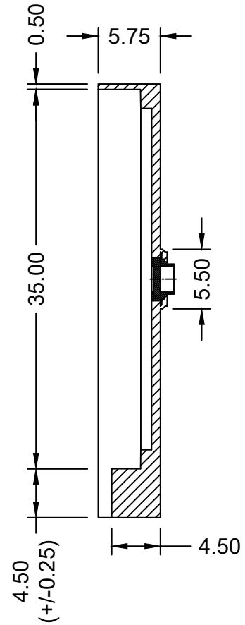
SECTION B-B
