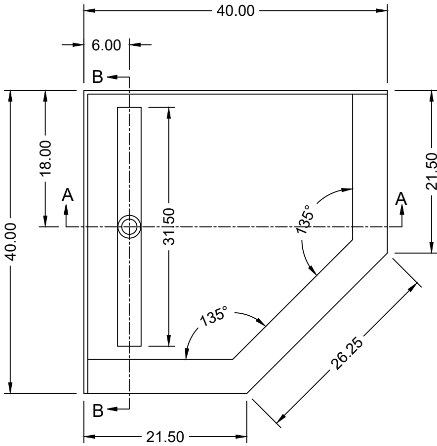
TOP VIEW
