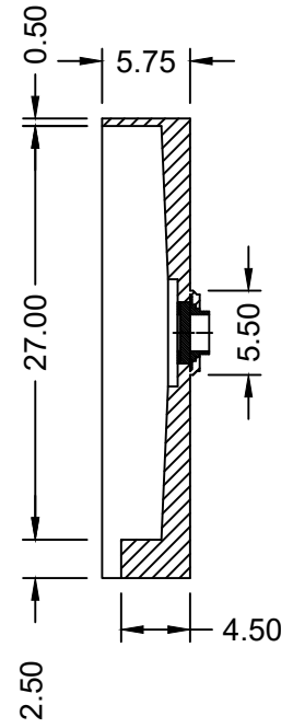
SECTION B-B
