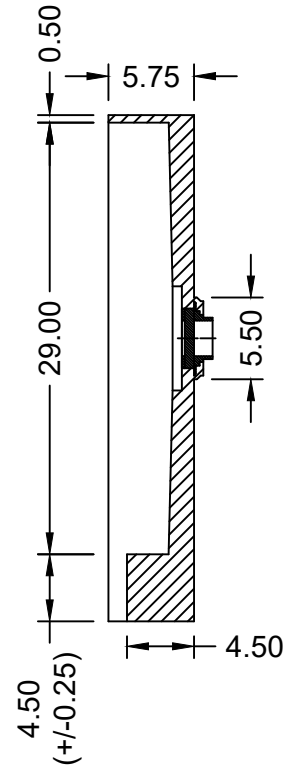
SECTION B-B
