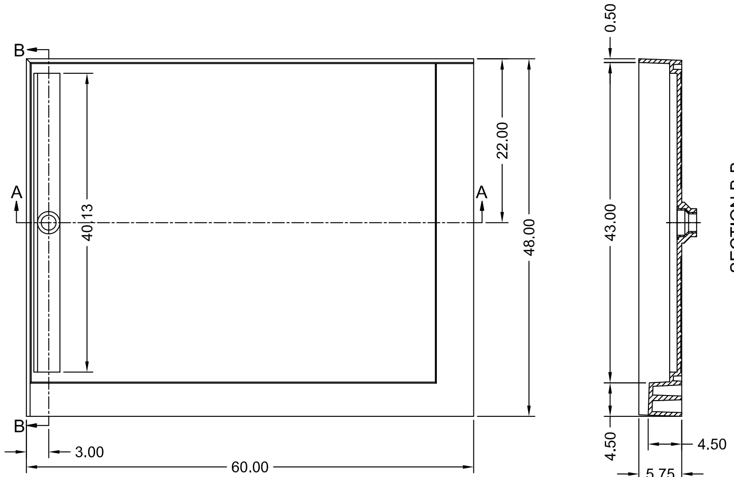
SECTION B-B
