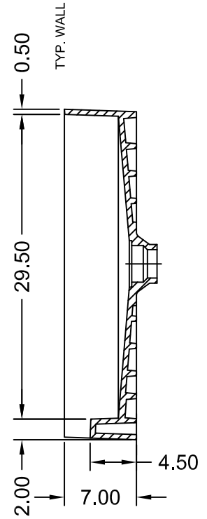
SECTION B-B
