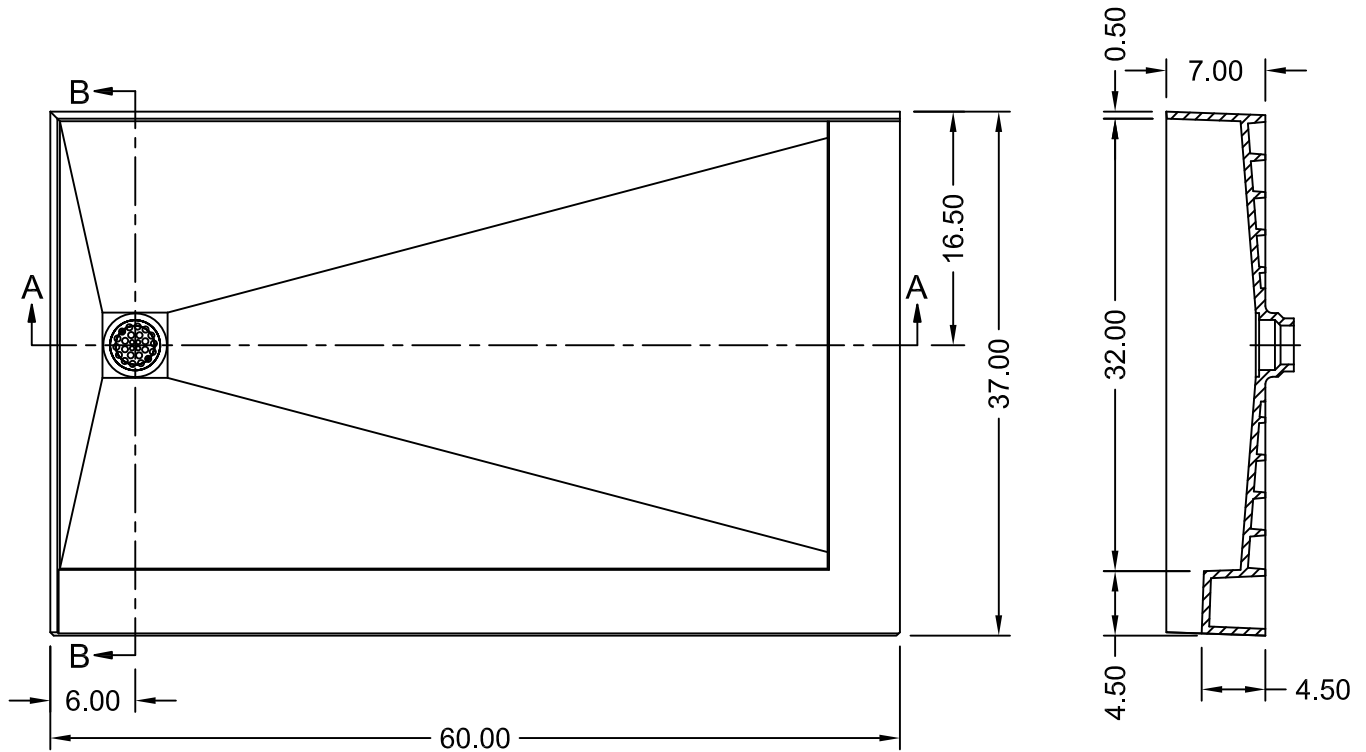
SECTION B-B
