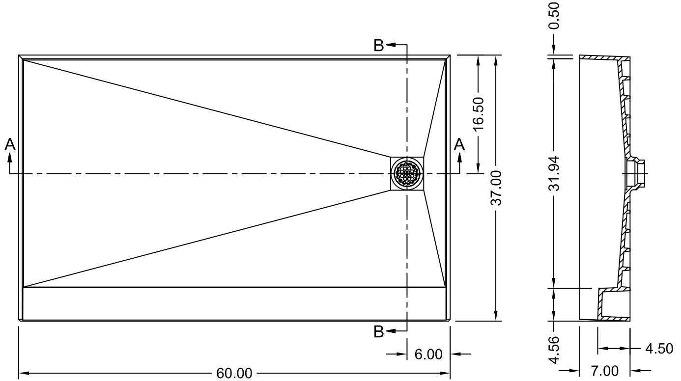
SECTION B-B
