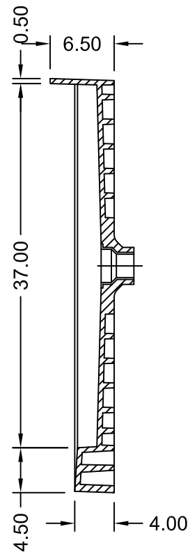
SECTION B-B
