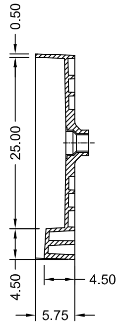
SECTION B-B
