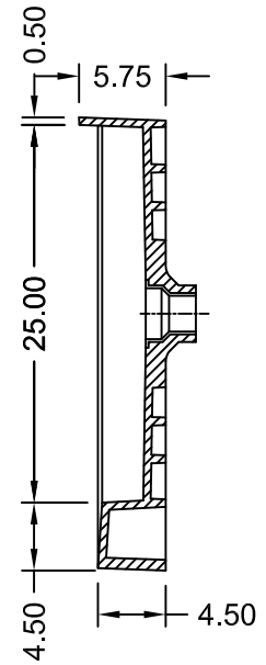
SECTION B-B
