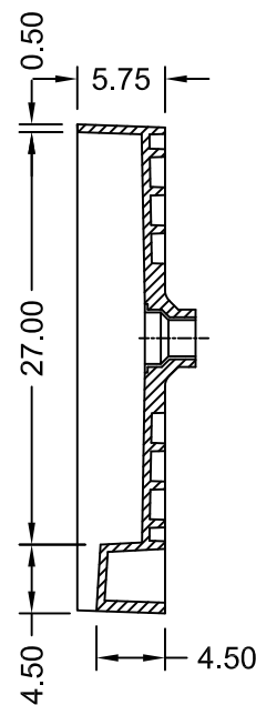
SECTION B-B
