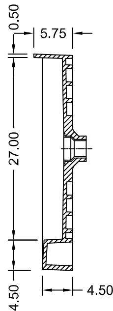
SECTION B-B
