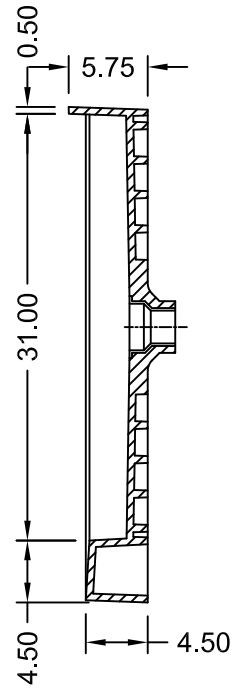
SECTION B-B
