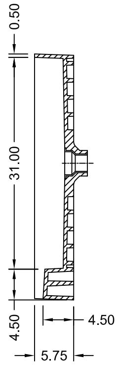
SECTION B-B
