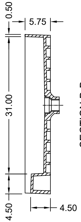
SECTION B-B
