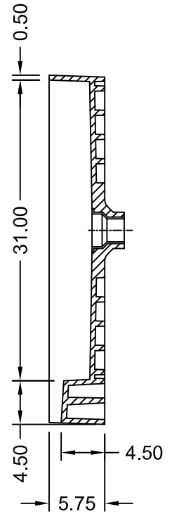
SECTION B-B
