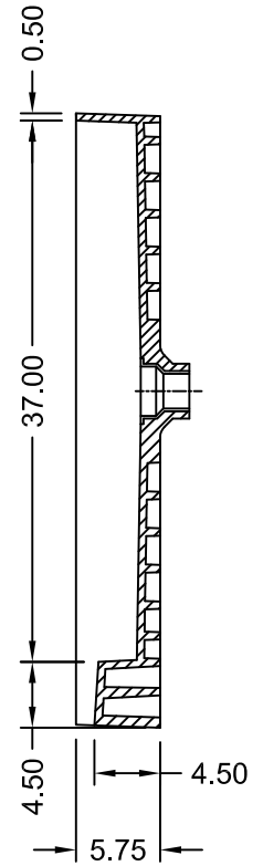
SECTION B-B
