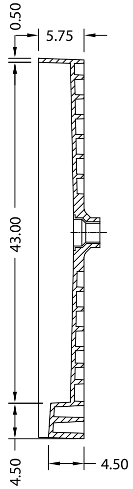
SECTION B-B
