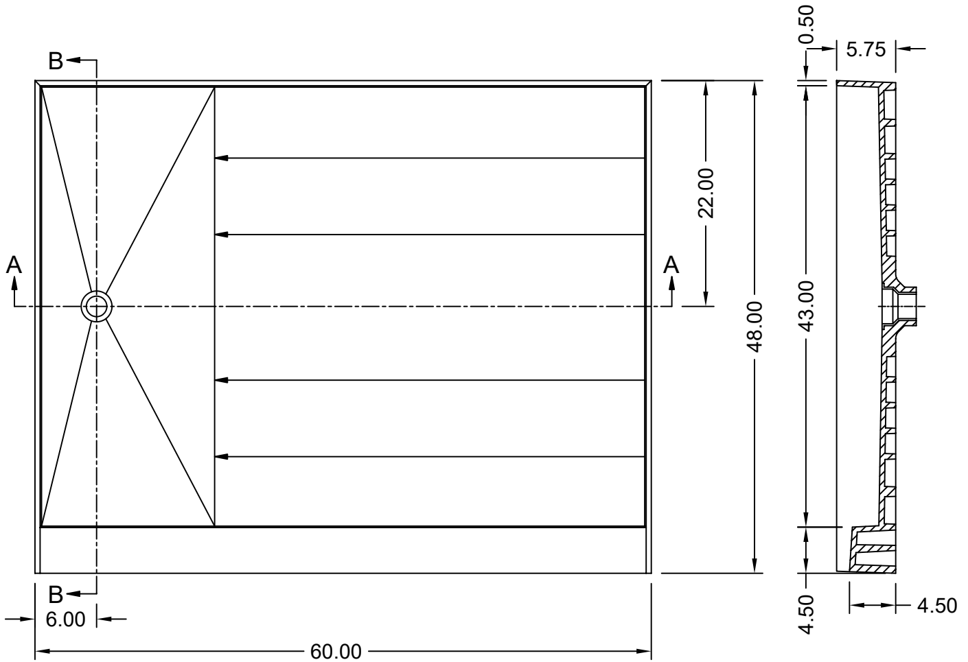
SECTION B-B
