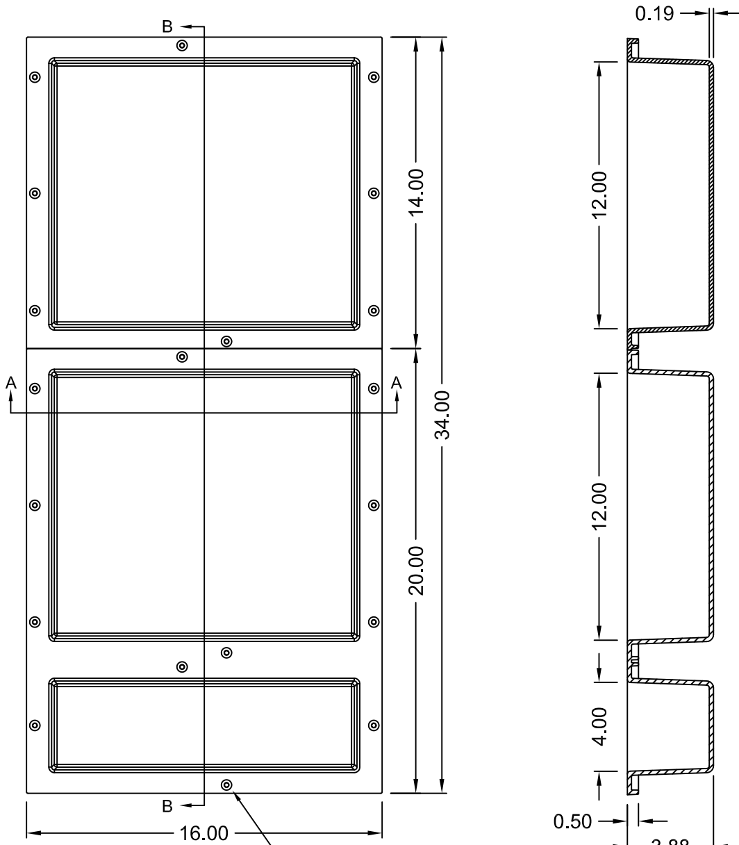
SECTION B-B
