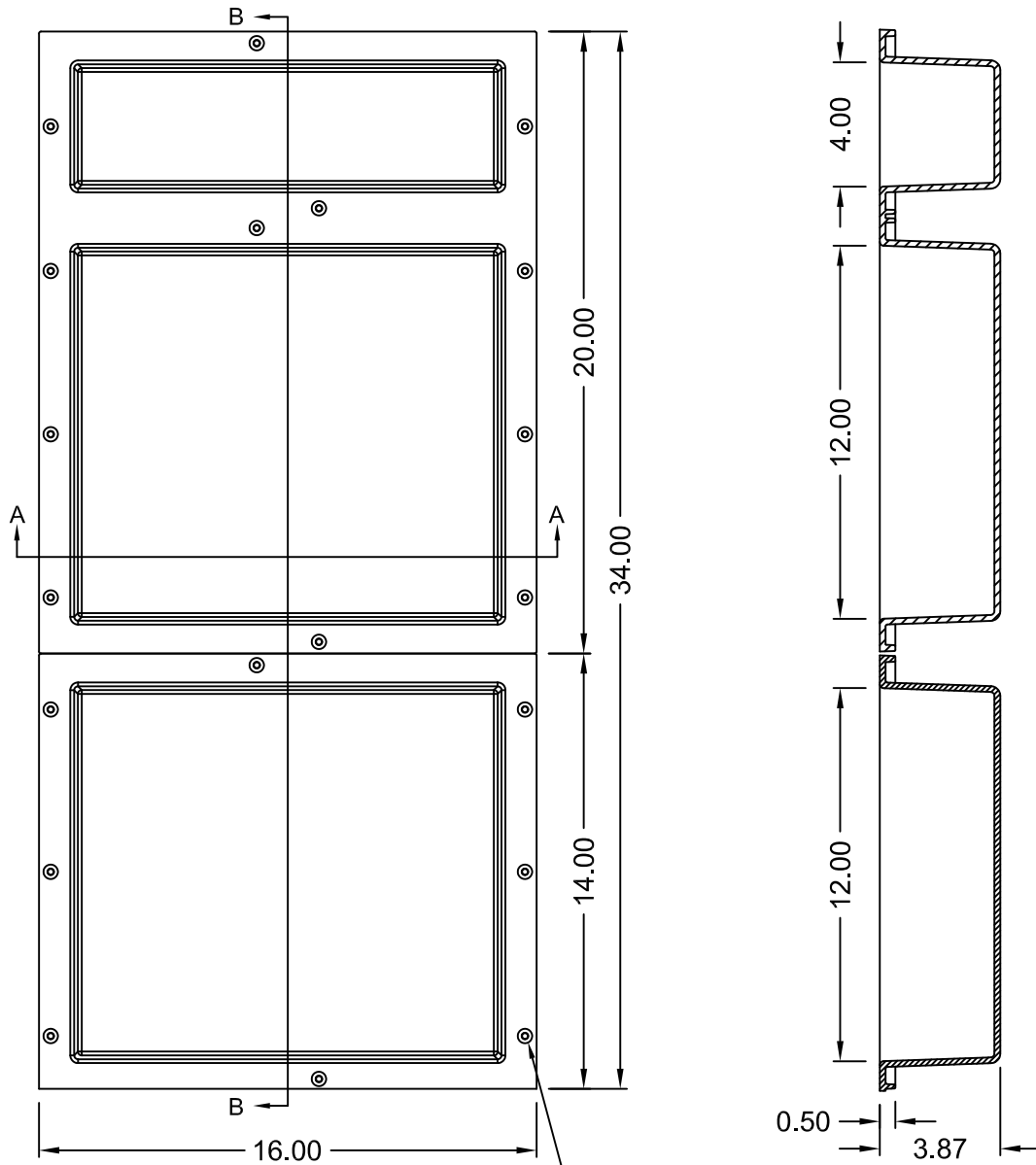
SECTION B-B
