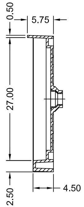
SECTION B-B
