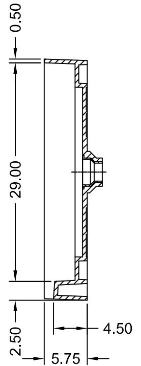
SECTION B-B
