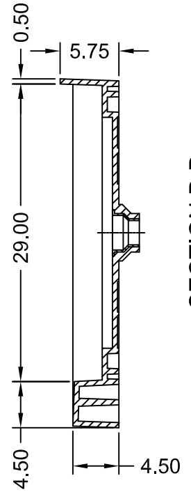
SECTION B-B
