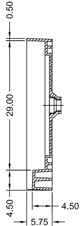
SECTION B-B
