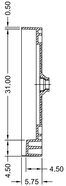
SECTION B-B
