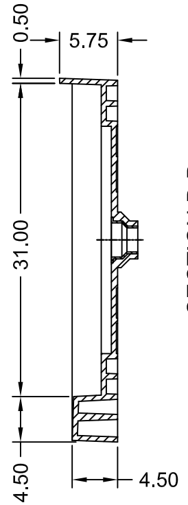
SECTION B-B
