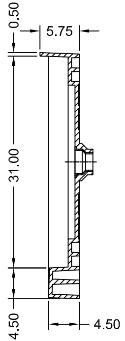
SECTION B-B
