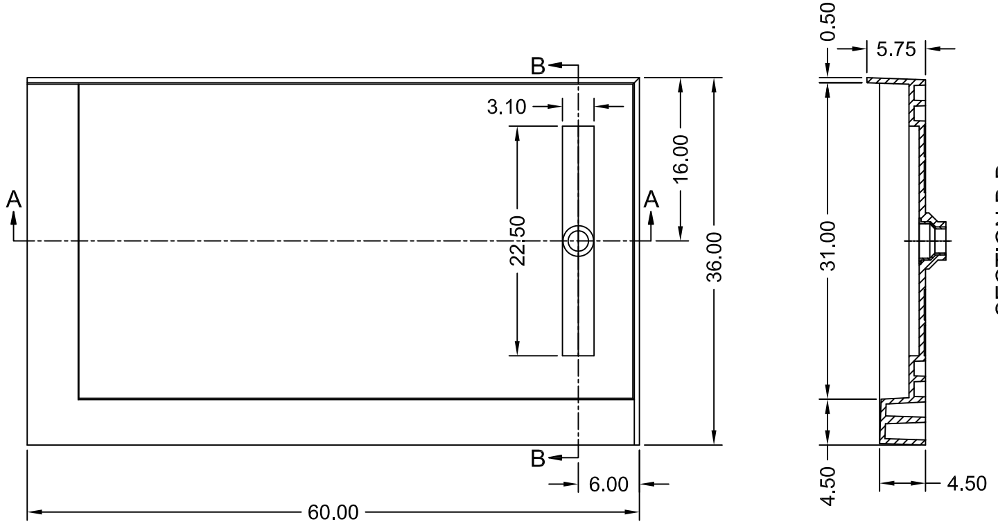
SECTION B-B
