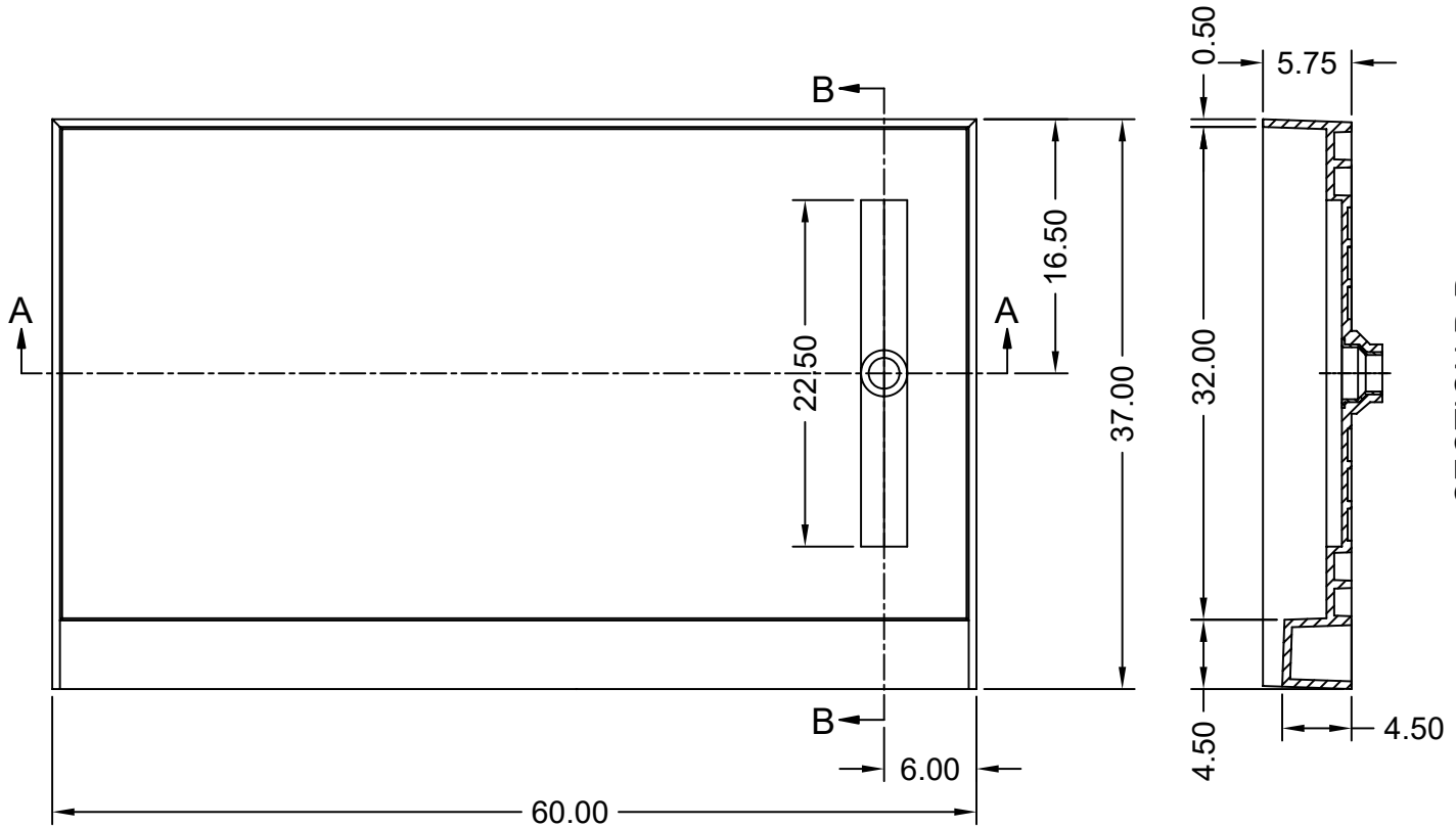
SECTION B-B
