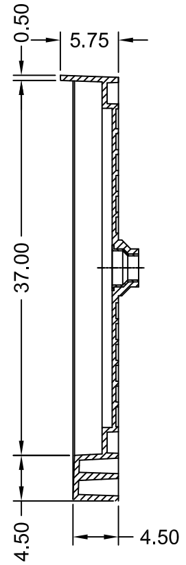
SECTION B-B
