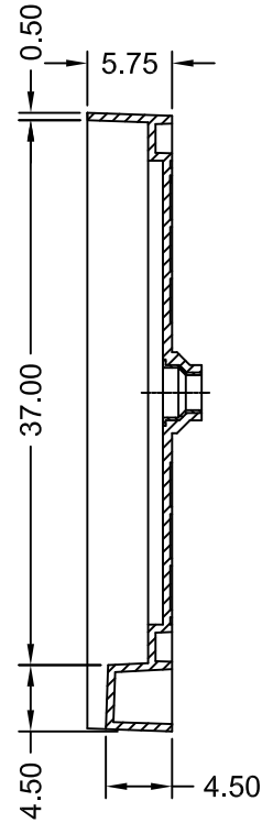
SECTION B-B
