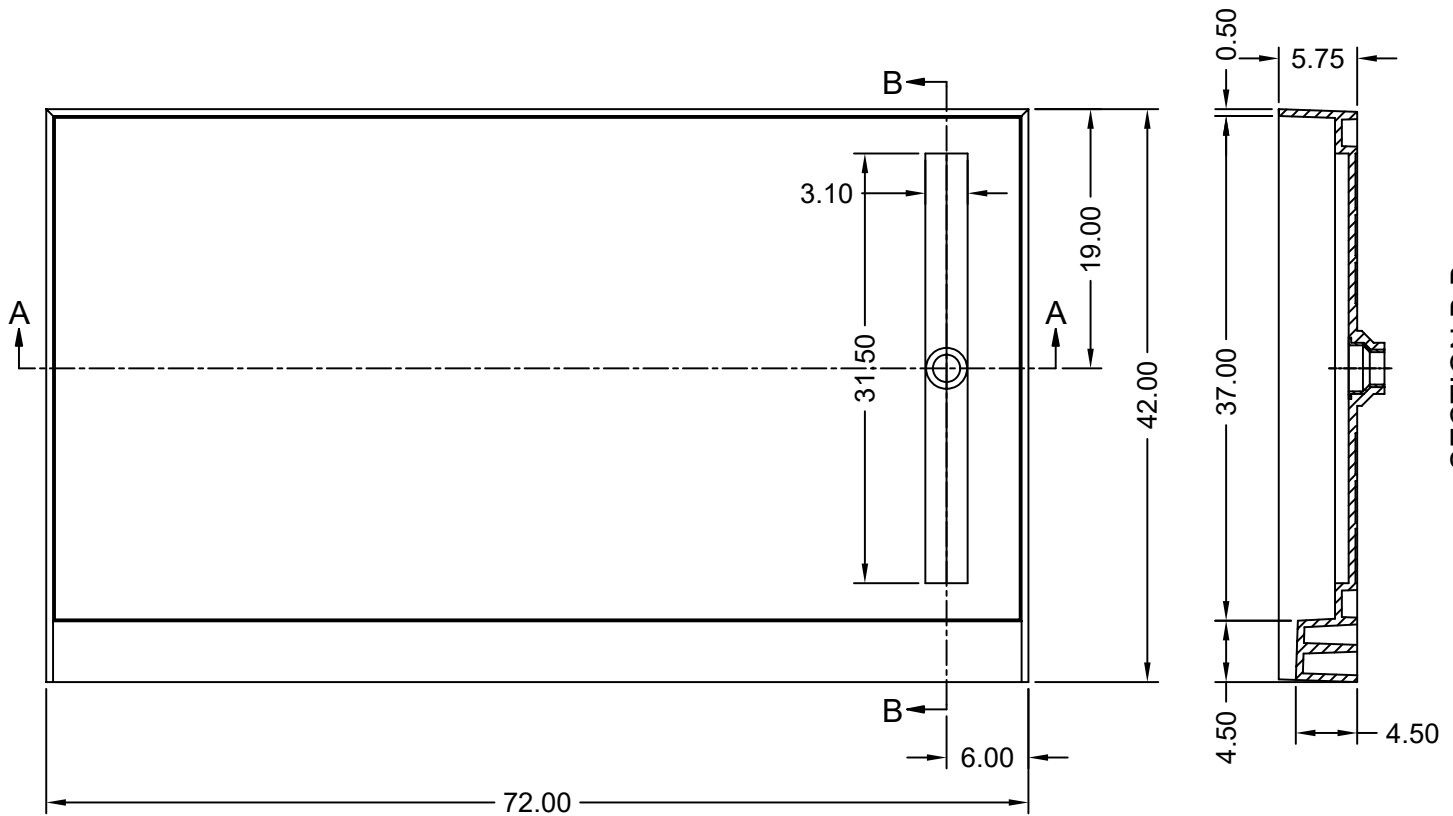
SECTION B-B
