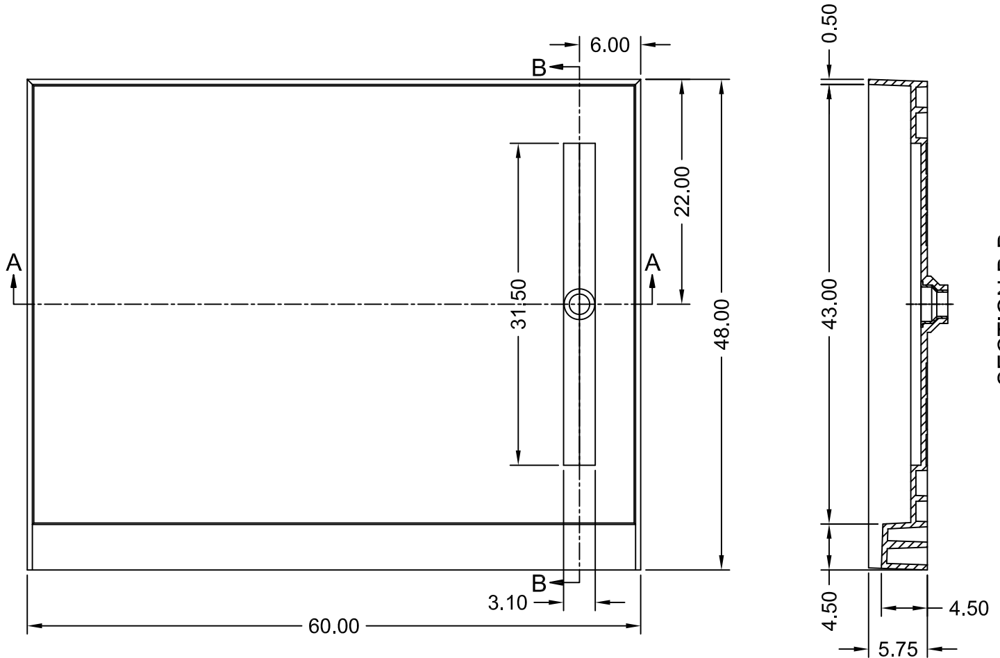
SECTION B-B
