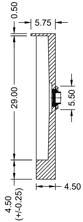
SECTION B-B
