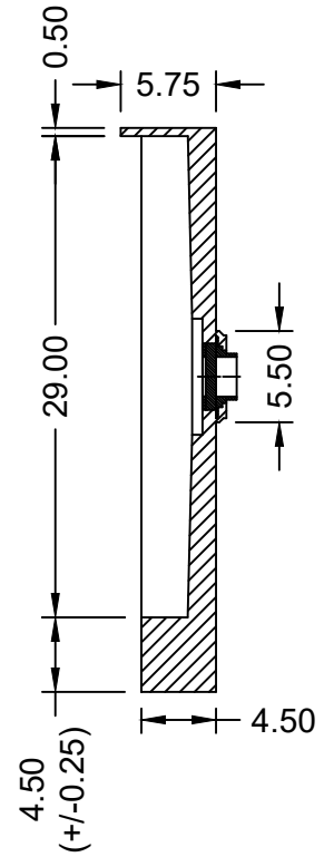
SECTION B-B
