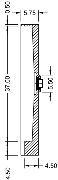
SECTION B-B
